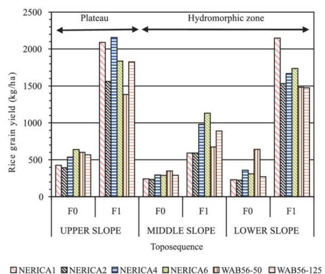
Yield benefit of NERICA lines along topographic gradient (F0: unfertilized, F1: fertilized).
